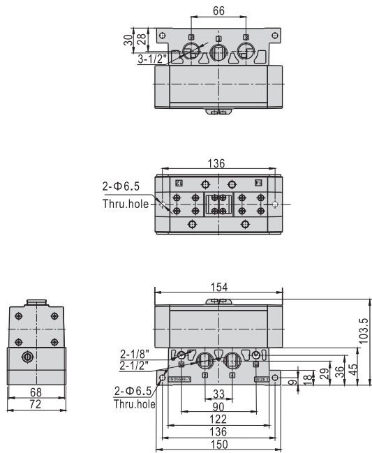
EAV430+ESV401M
