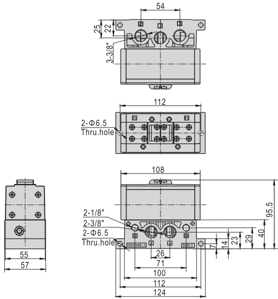
EAV310/320+ESV301M
